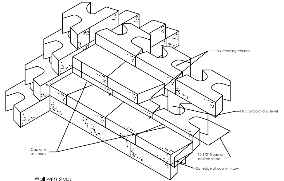
Wall with Steps With full blocks and universal caps
